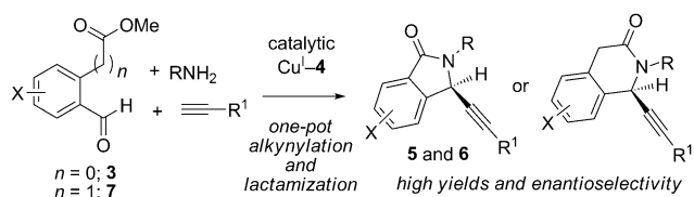
Scheme 2. Proposed copper(I)-catalyzed alkynylation/lactamization cascade.
